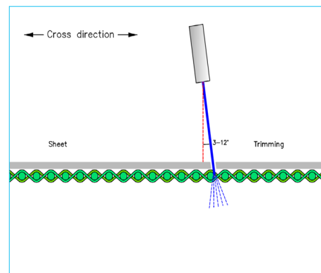
Fig. 14 Water jet diagonal in cross direction
